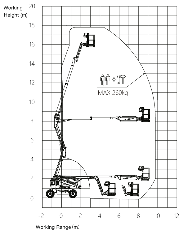
LA16JE Performance Curve
