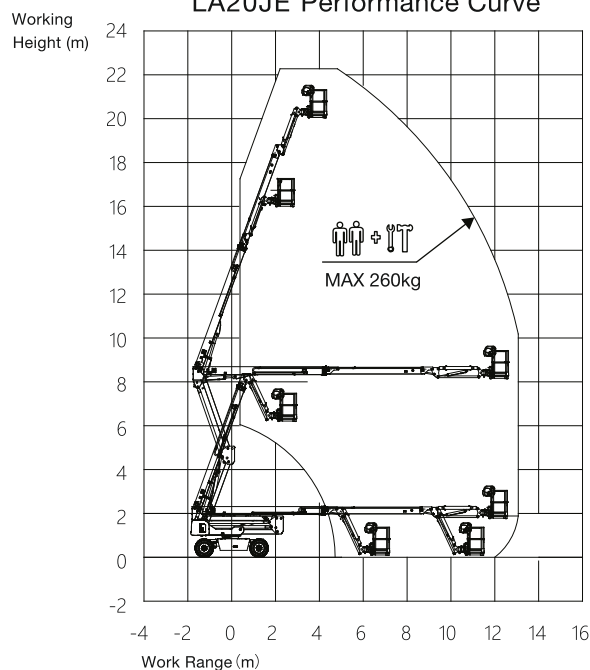
LA20JE Performance Curve
